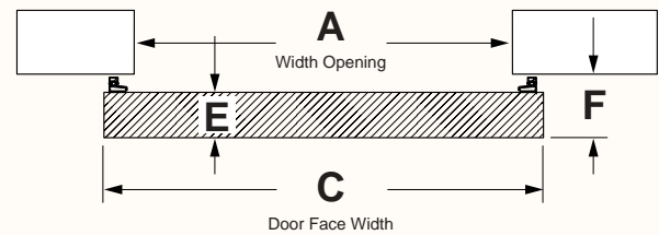
Overlap / Slab Type Door
