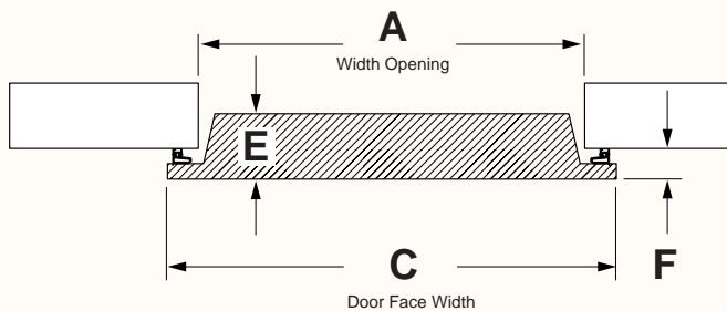
Infitting Type Door
